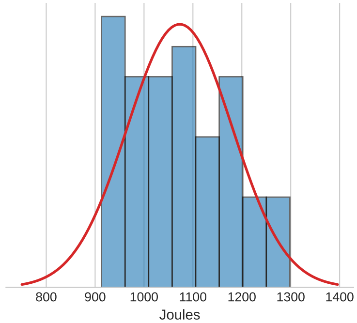
Statistical Distribution
