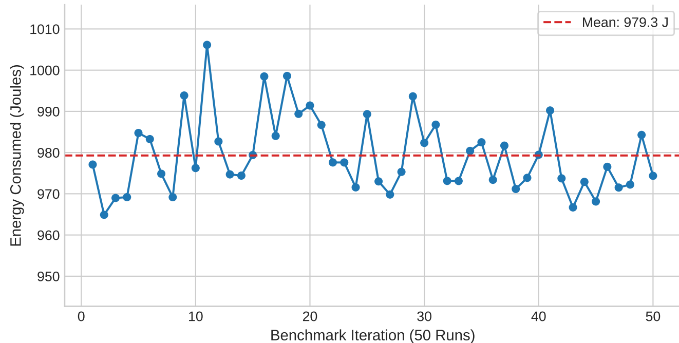
CPU Package Energy (Baseline Stability)
