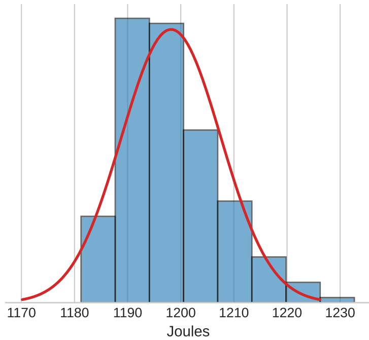
Statistical Distribution
