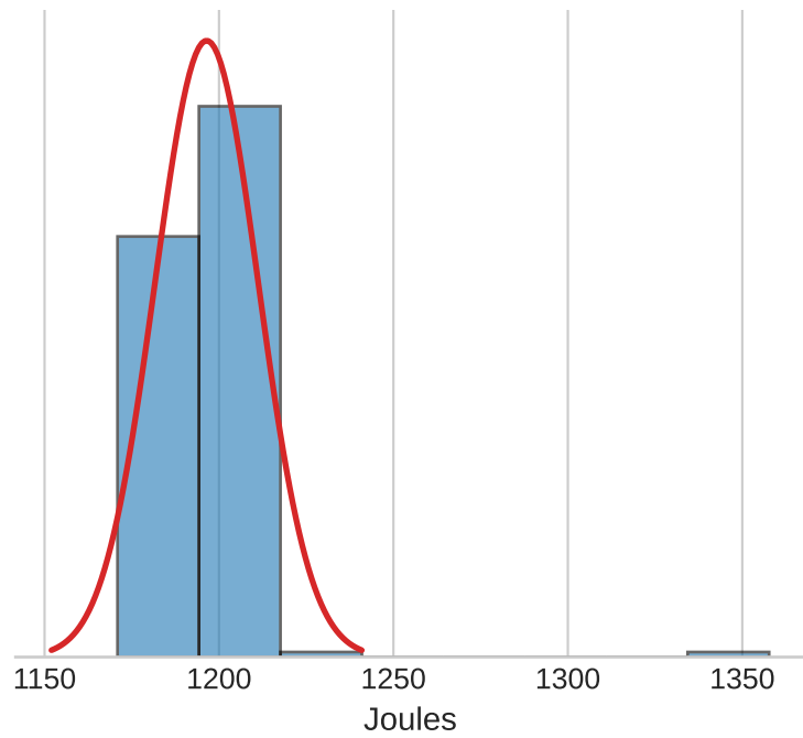
Statistical Distribution
