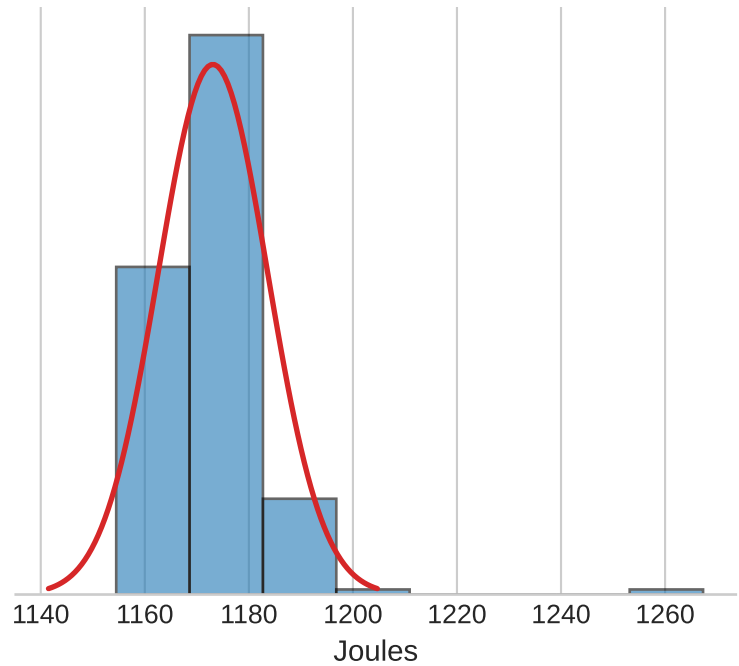
Statistical Distribution
