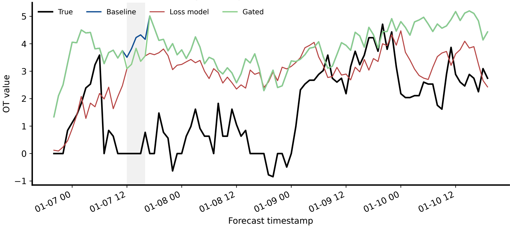
GPT-5.5 Long-tail Region 1: window 1796, channel OT
