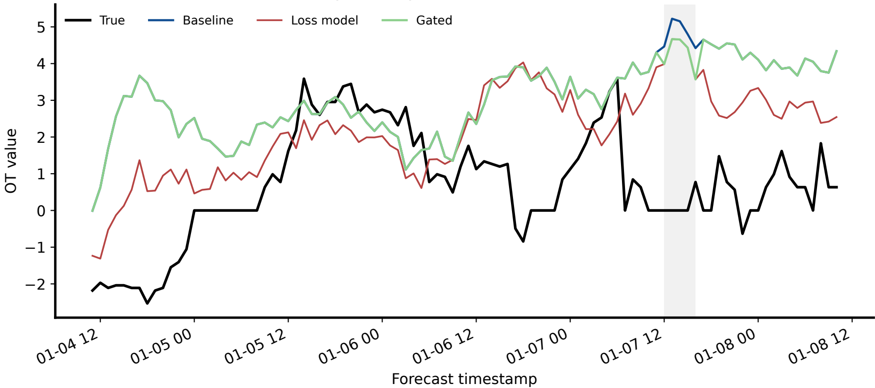
GPT-5.5 Long-tail Region 3: window 1739, channel OT
