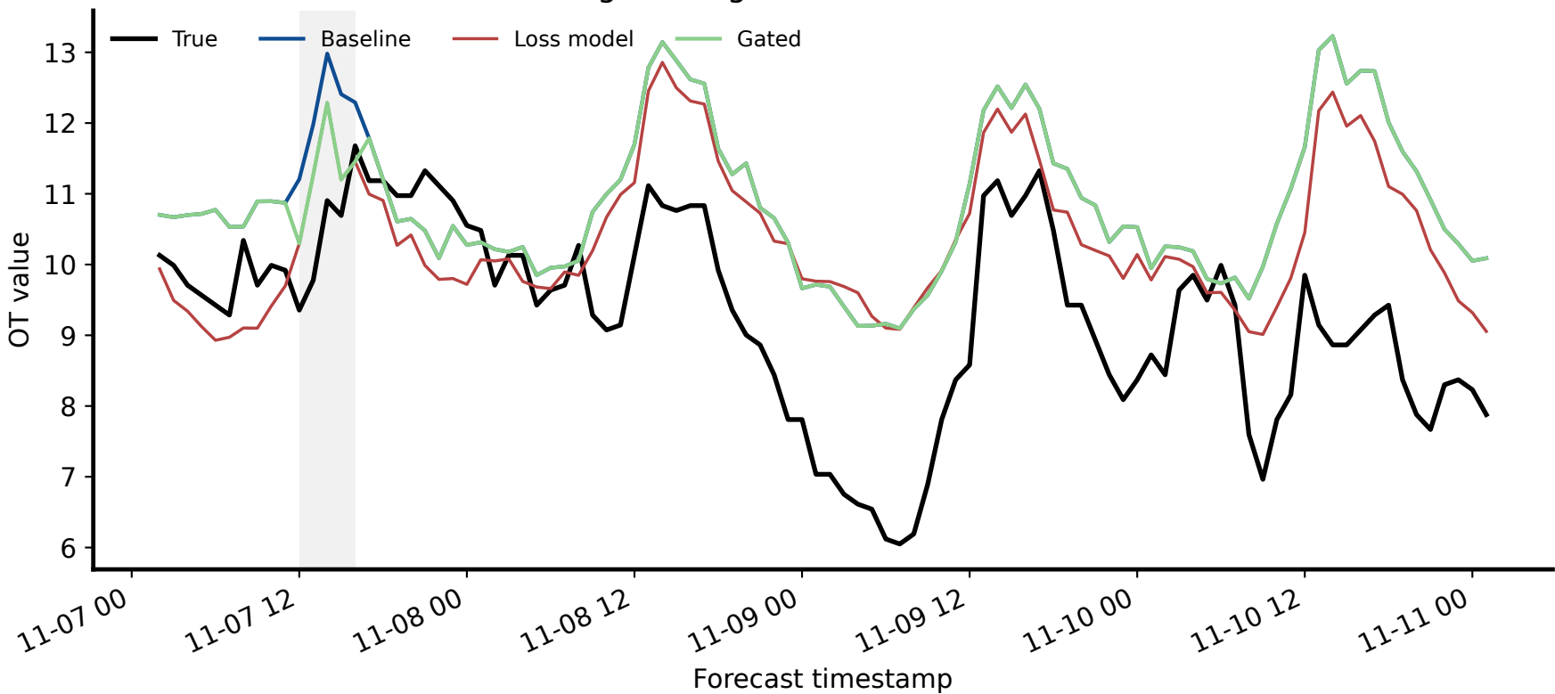
GPT-5.5 Long-tail Region 4: window 338, channel OT
