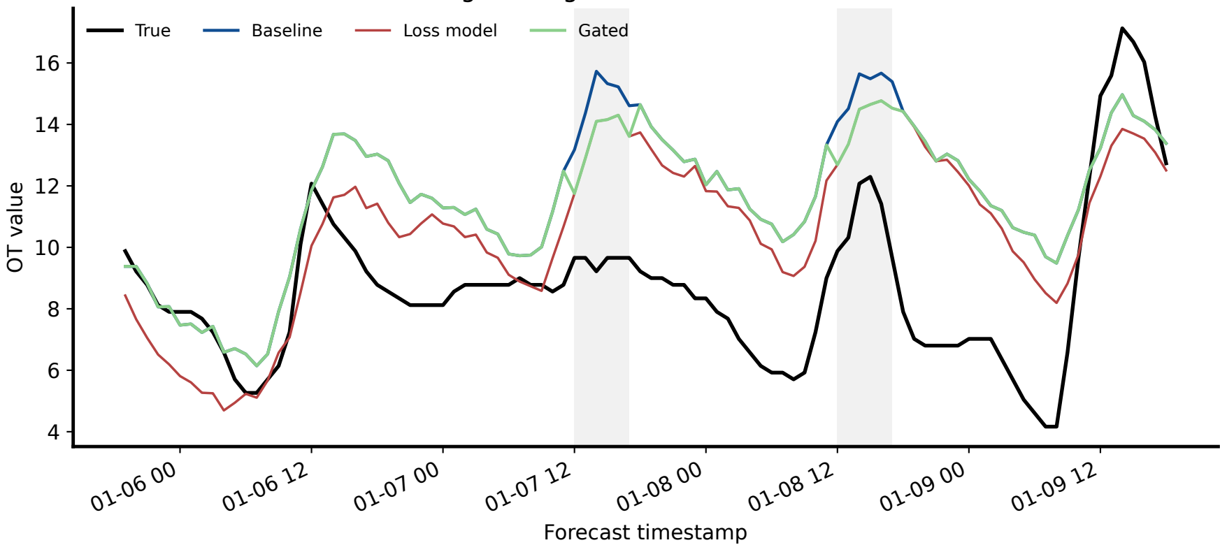
GPT-5.5 Long-tail Region 2: window 1771, channel OT
