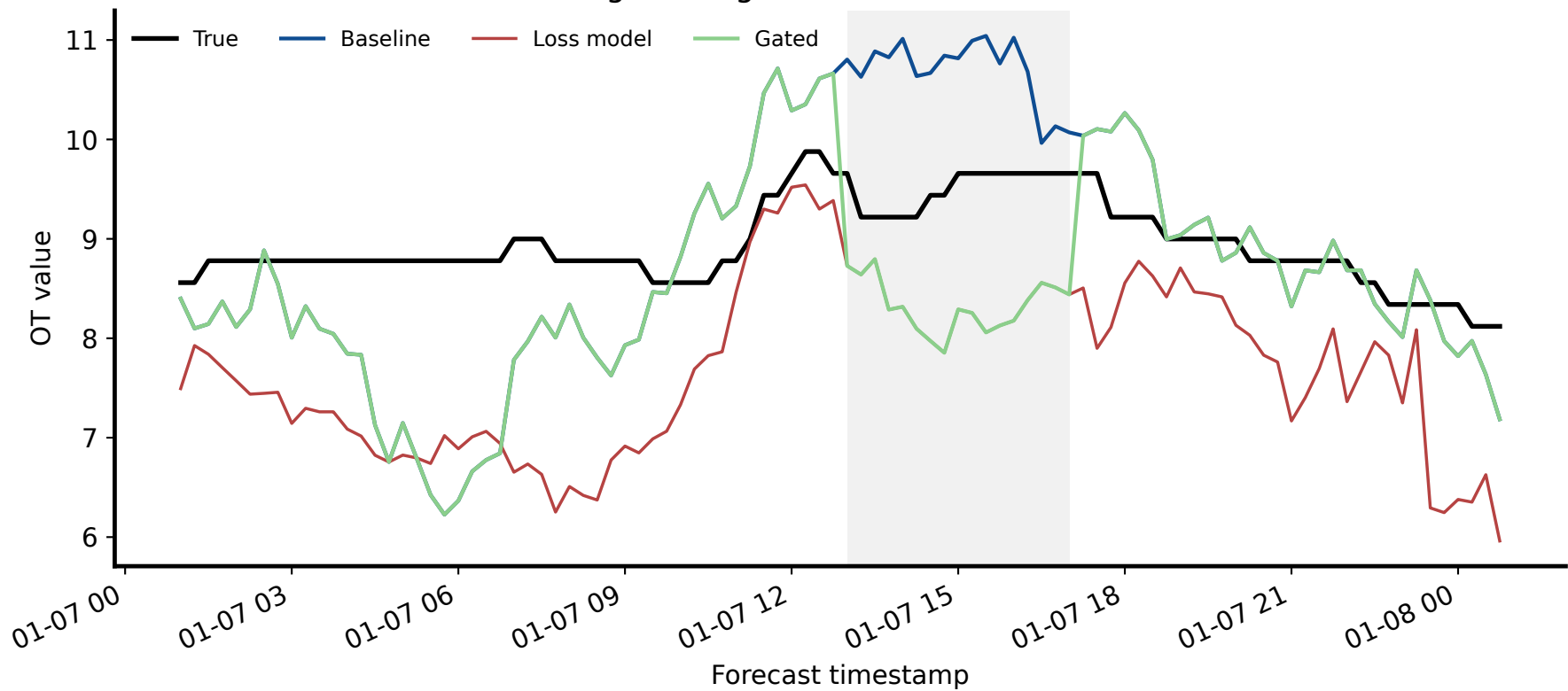
GPT-5.5 Long-tail Region 1: window 7204, channel OT
