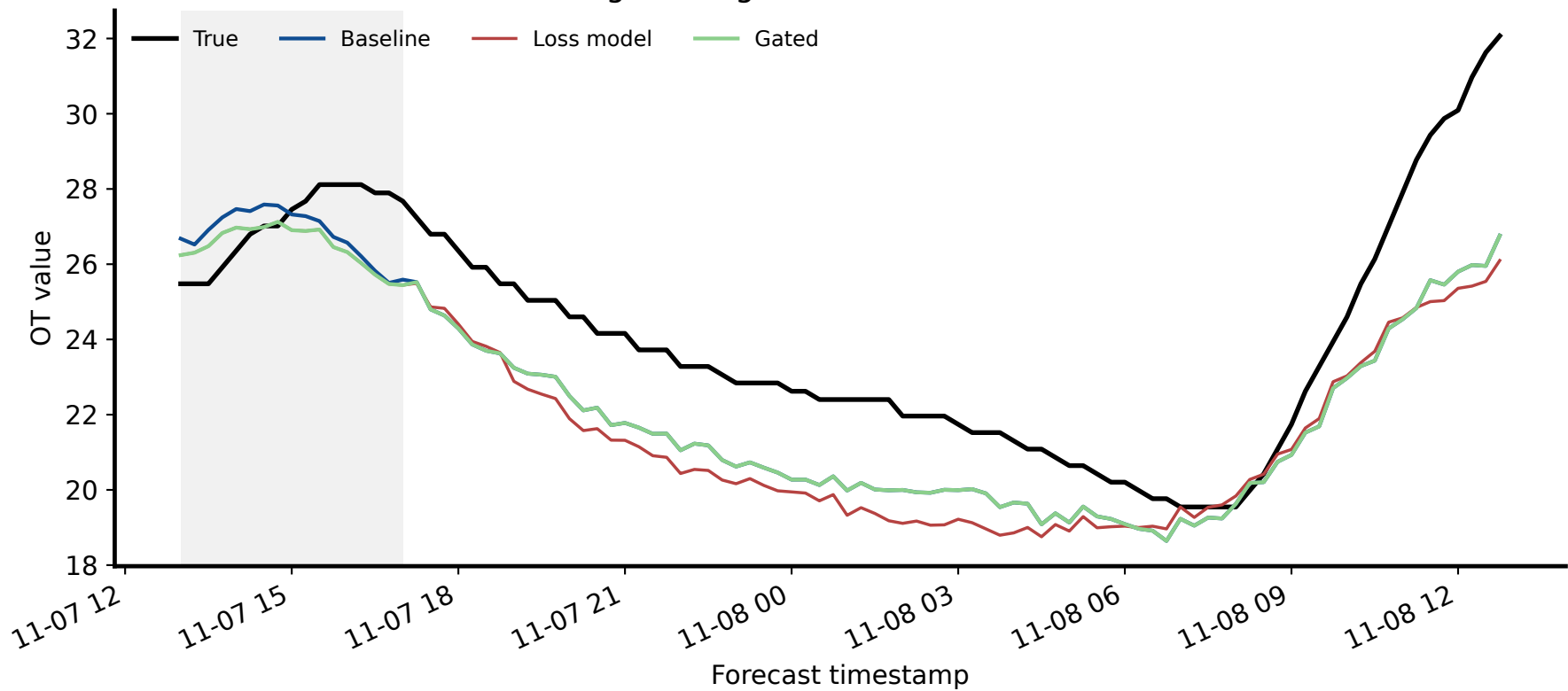
GPT-5.5 Long-tail Region 4: window 1396, channel OT
