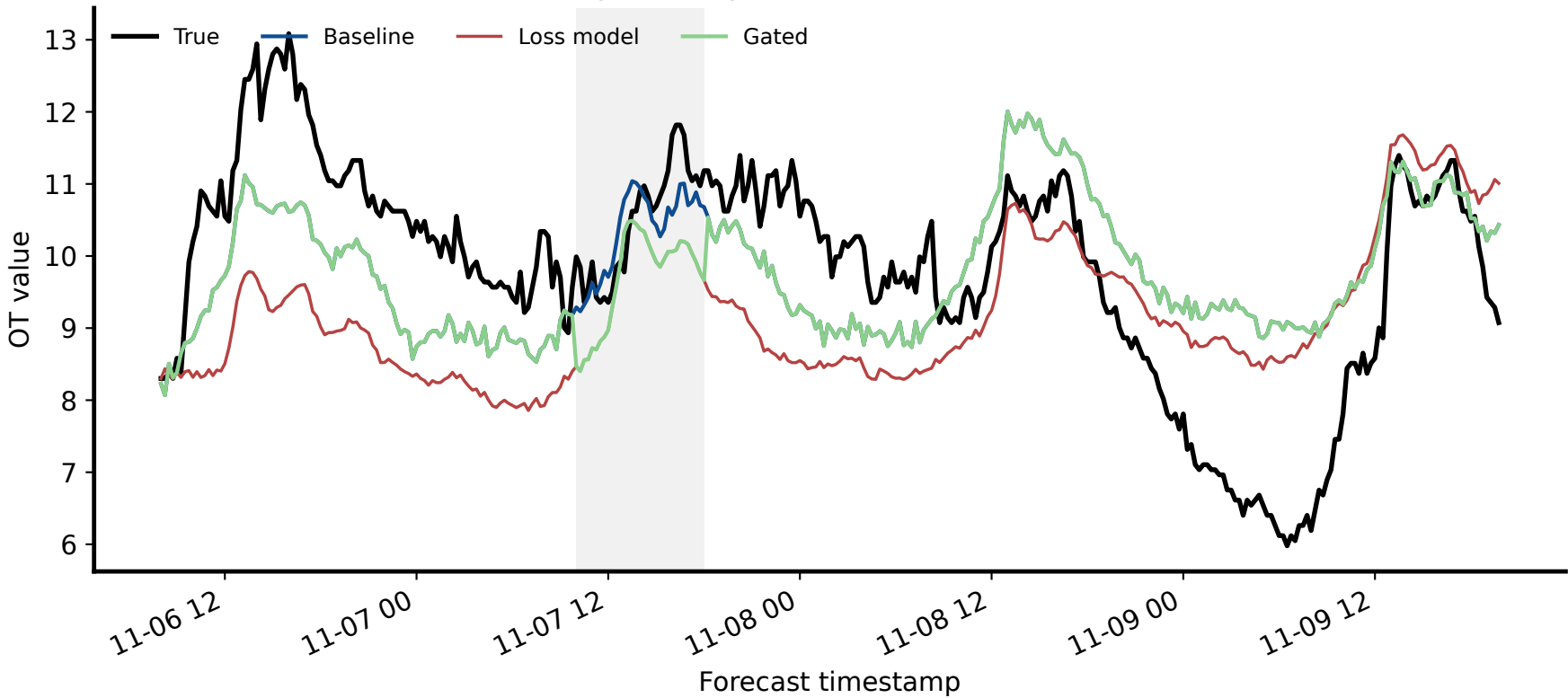
GPT-5.5 Long-tail Region 1: window 1280, channel OT
