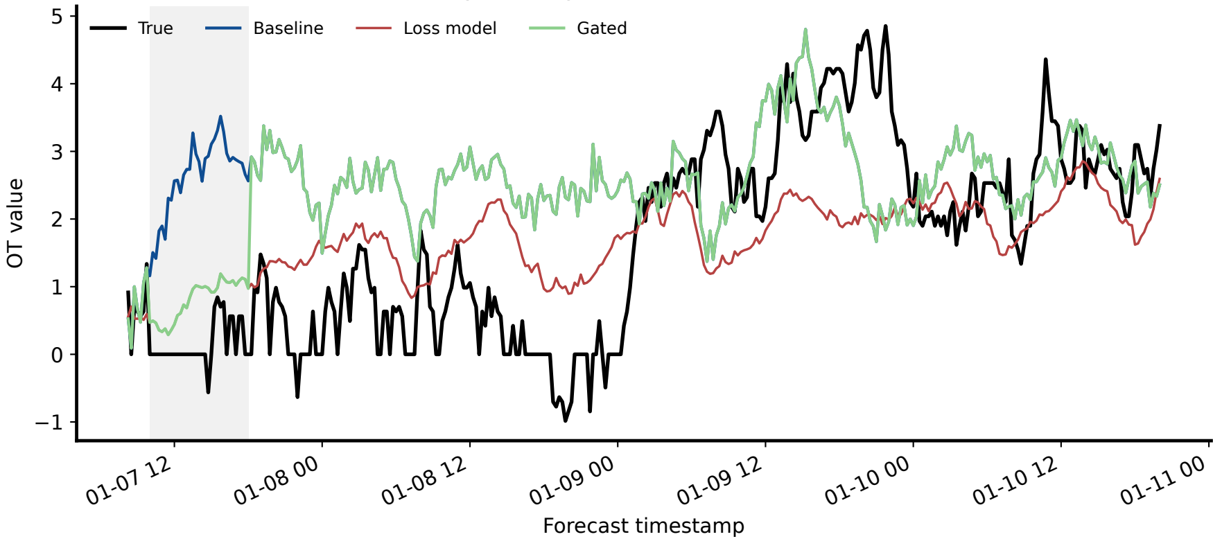
GPT-5.5 Long-tail Region 3: window 7233, channel OT
