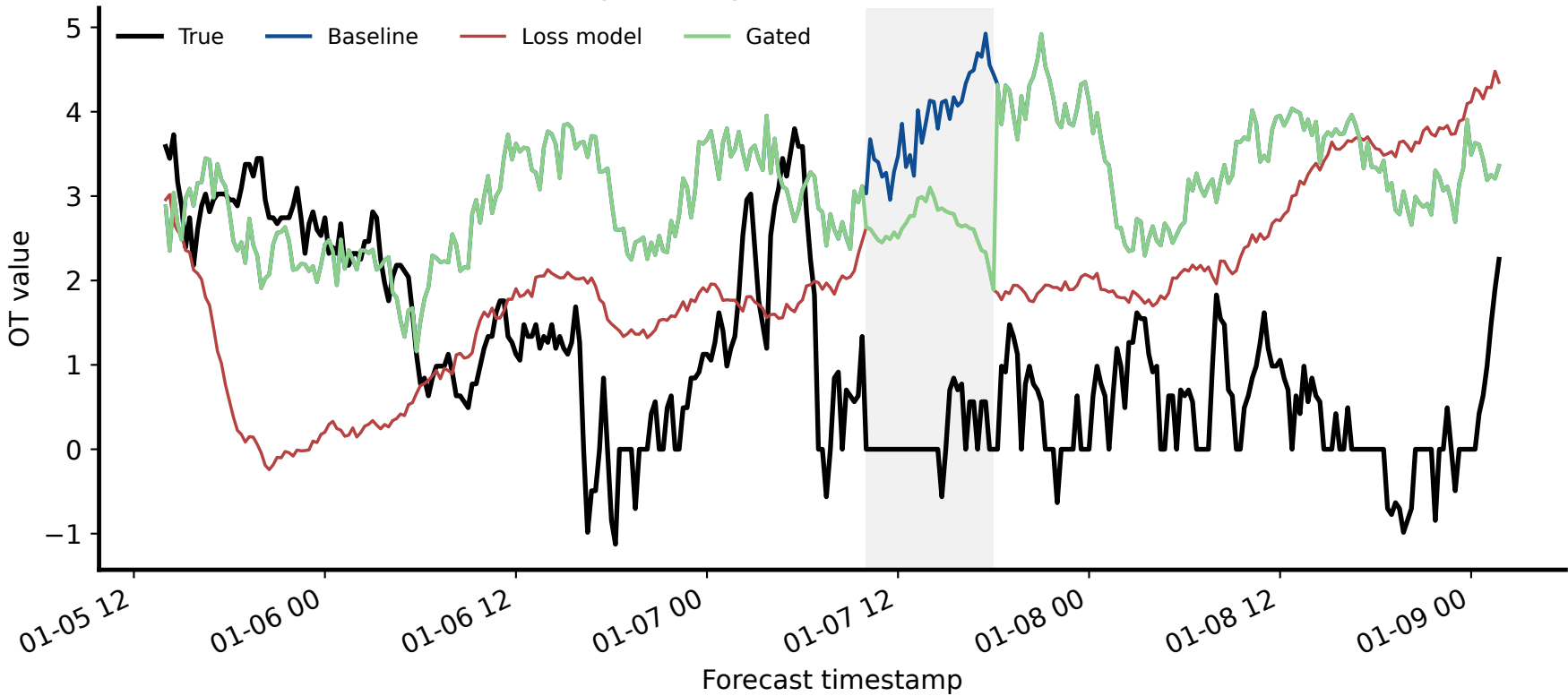
GPT-5.5 Long-tail Region 4: window 7064, channel OT
