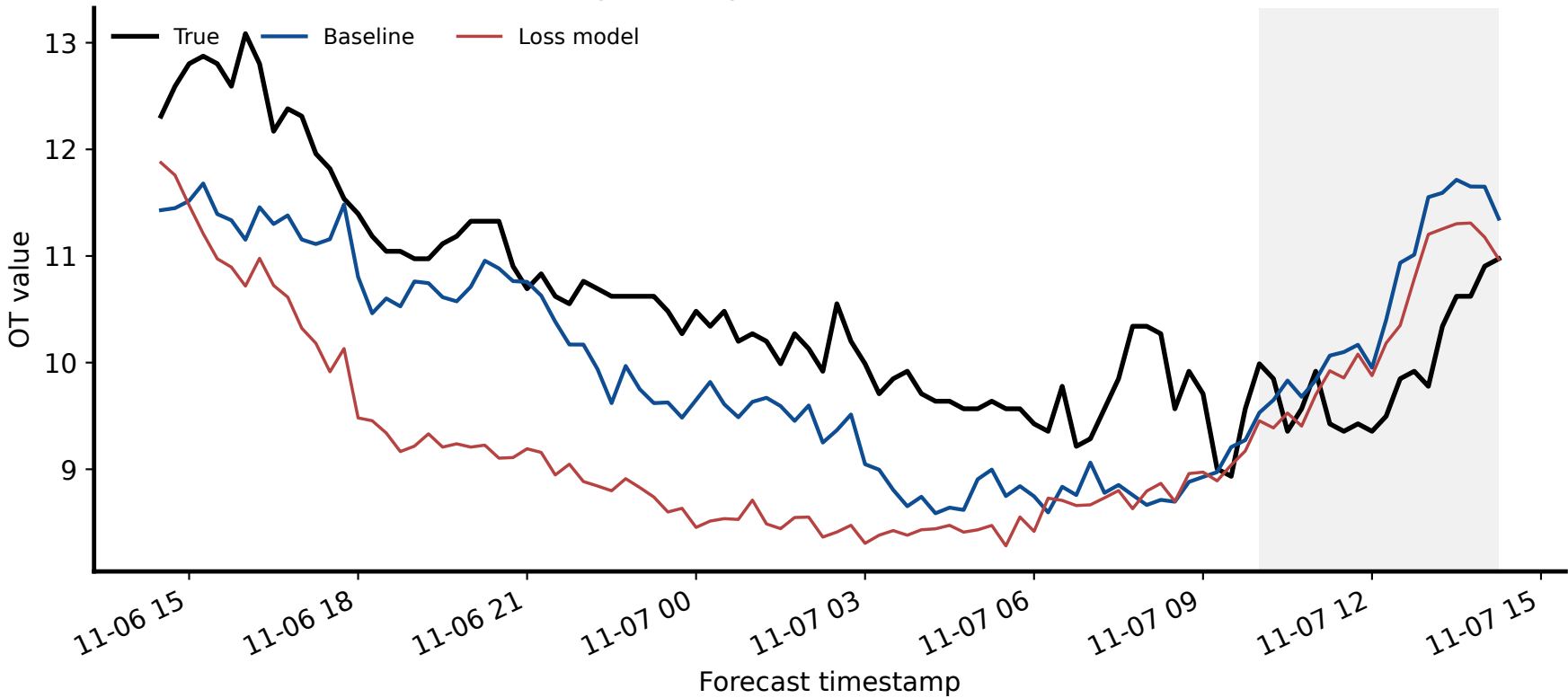
GPT-5.5 Long-tail Region 4: window 1306, channel OT
