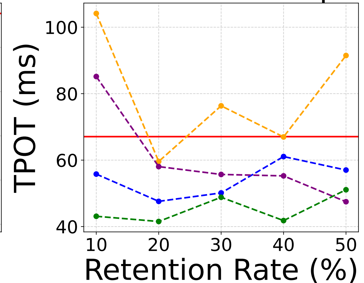
TPOT on ActCap
