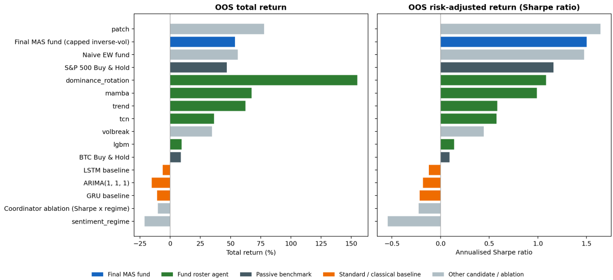
Figure 6.5: Ranked OOS total return (left) and annualised Sharpe ratio (right), with bars coloured by role (legend): the final fund (blue), the five fund-roster agents (green), the passive benchmarks (slate), the standard recurrent and classical baselines (orange, GRU/LSTM and ARIMA), and the remaining candidates and ablations (grey). On total return the fund sits mid-pack — by construction, since diversification trades peak return for stability — but on risk-adjusted return it ranks first among the roster agents and benchmarks (the only higher Sharpe, the excluded PatchTST, is skill-free bear beta), while the GRU, LSTM and ARIMA baselines sit together at the negative-Sharpe bottom of the ranking.
