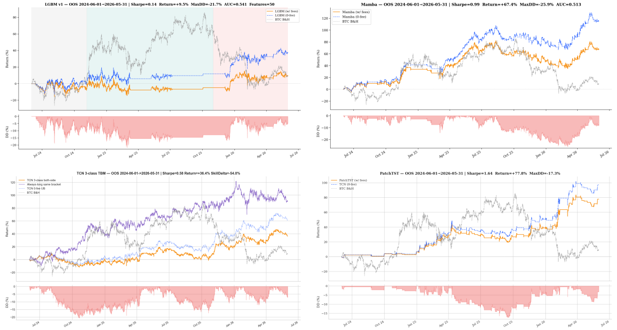
Figure 6.2: Out-of-sample equity and drawdown for the four learned agents, each running its own frozen ATR-bracket strategy: LightGBM and Mamba (top, realised long-only over OOS), TCN and PatchTST (bottom, two-sided and short-only respectively). LightGBM, Mamba and TCN enter the fund; PatchTST is shown for comparison but is screened out (no out-of-sample directional skill). The curves are visibly dissimilar — different entry timing, different drawdown structure — which is the kind of decorrelation the fund allocator exploits among the agents it retains.
