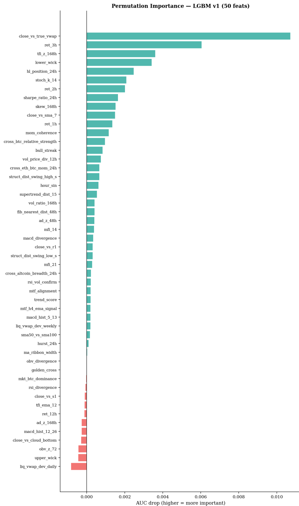
Figure 6.3: Permutation importance for the final LightGBM model on the OOS window. The small magnitudes are consistent with weak but non-zero hourly predictability: no single technical indicator dominates, and the selected feature set mixes price location, short-horizon momentum, flow, wick structure, and cross-asset context.
