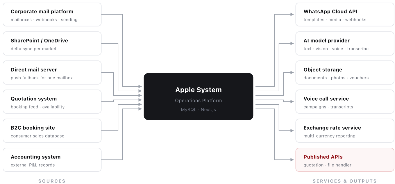
Figure 12.1 — The integration map. Six inbound systems, five outbound services, and two APIs the platform itself publishes for other applications to call.
