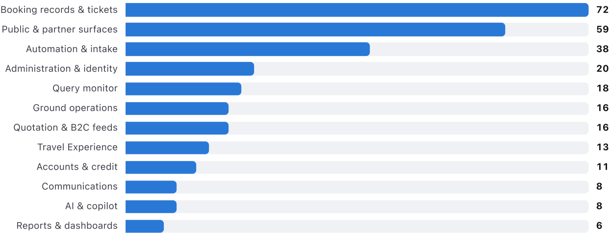
Figure A.1 — Endpoint count by functional domain, summing to the platform's 285 routes. Every endpoint runs the same three checks described in Part 4.
