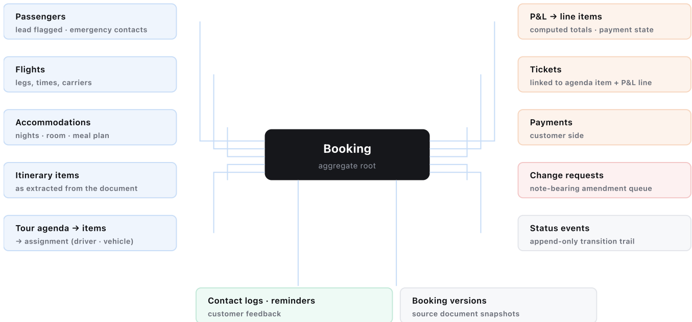
Figure 13.1 — The booking aggregate. A ticket deliberately links to both its agenda item and its P&L line, which is what keeps the operational and financial views of the same purchase from ever drifting apart.
