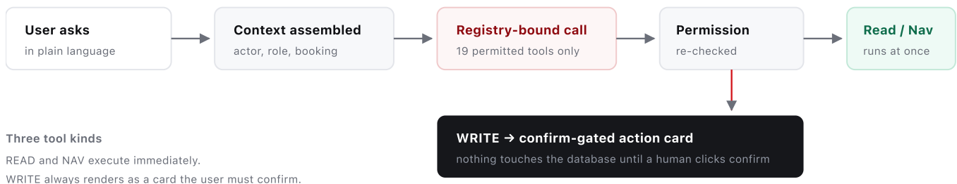
Figure 10.1 — The copilot request flow. Proposing an action is the permission request — which is why the assistant never needs to ask "shall I?" in prose.
