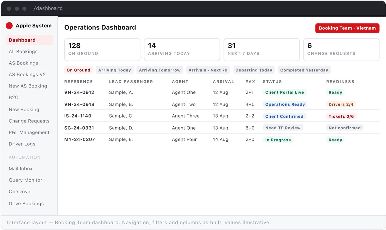
Figure 5.1 — The dashboard shell. The sidebar shown is the Booking Team's; each role receives a different one generated from its permission set.
