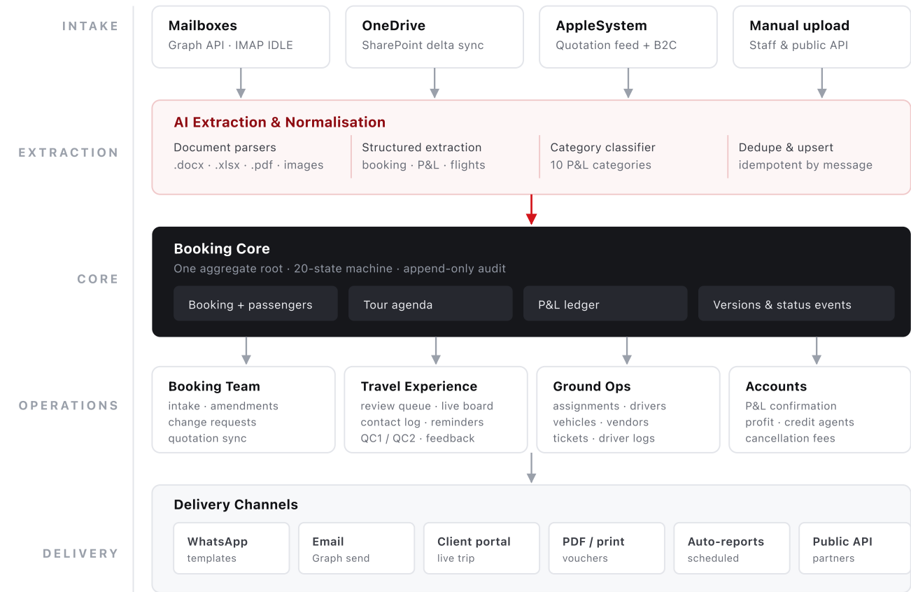
Figure 2.1 — The five architectural layers. All four intake channels converge on a single extraction path, so a booking created from a mailbox is indistinguishable downstream from one created by hand or pulled from the quotation feed.
