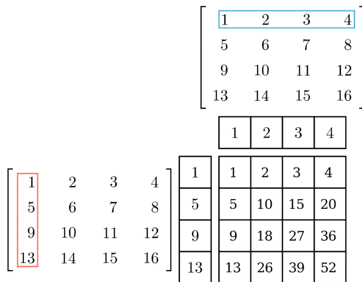
Abbildung 5.2: Matrix Engine
