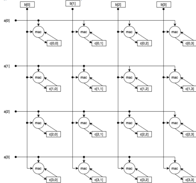
Abbildung 2.6: Matrix Accumulator (MAC)
