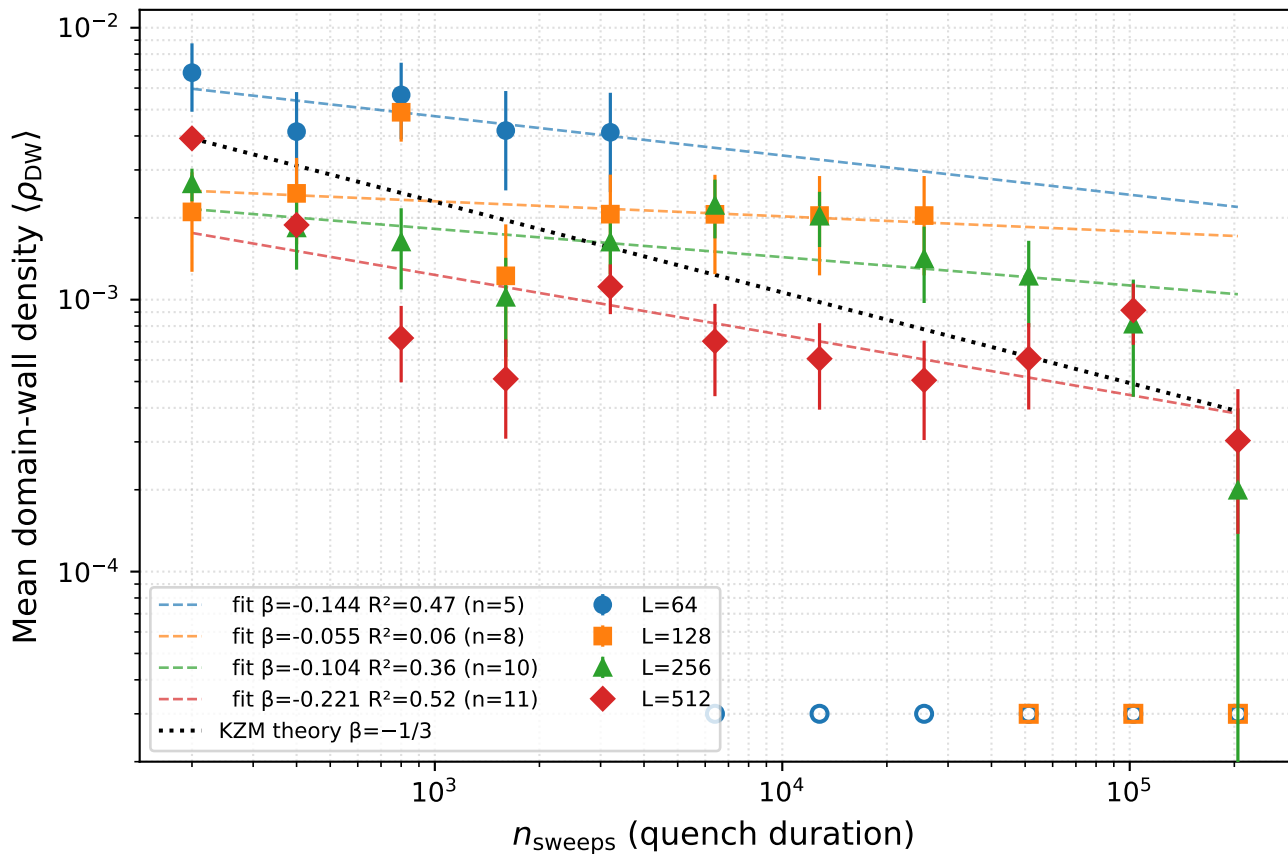
Exp 107 — KZM Scaling: 2D AF Ising GPU (Checkerboard Metropolis)
