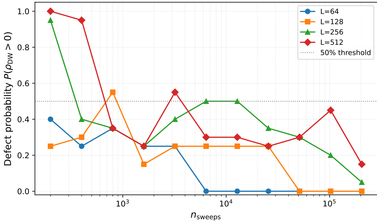
Exp 107 — Fraction of runs with \geq 1 domain wall
