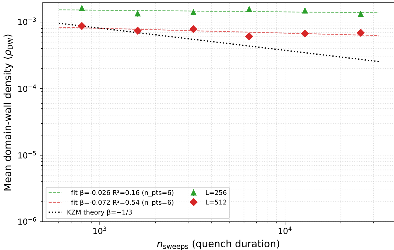
Exp 108 — KZM Scaling: Single-Wall Regime L \in \{256, 512\} , N = 200 reps, n \in [800, 25600]
