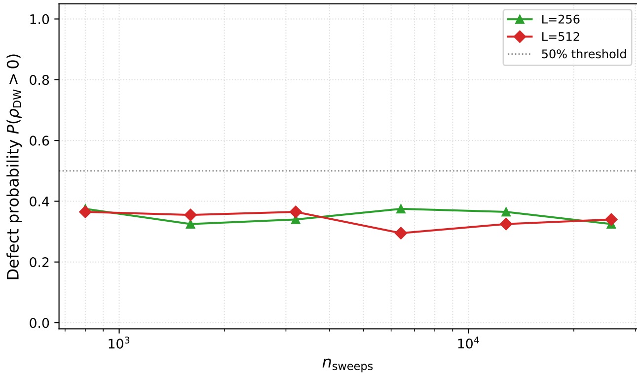
Exp 108 — Fraction of runs with \geq 1 domain wall
