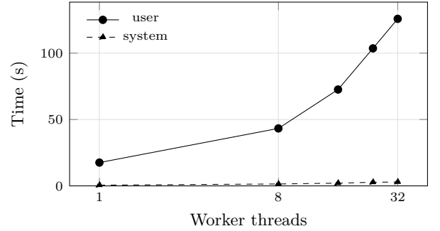
Figure 7: User and system time against worker count, for the runs of Table 13. Across a 32\times increase in workers user time rises by 7.2\times while system time rises by 5\times . System time is thirty to forty-five times the smaller and tracks the fault count. The efficiency decline of Figure 8 is spent in user time, on cross-domain data flow (Table 13’s section), with memory acquisition a minor kernel-side term.
