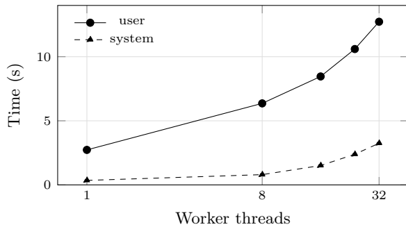
Figure 7: User and system time against worker count, for the runs of Table 14. Across a 32× increase in workers user time rises by 4.7× while system time rises by 9×. System time is the faster-growing term and it tracks the resident set: the kernel-side share of the efficiency decline of Figure 8 is memory acquisition rather than lock contention. The user-side share is cross-domain data flow (Table 14’s section).
