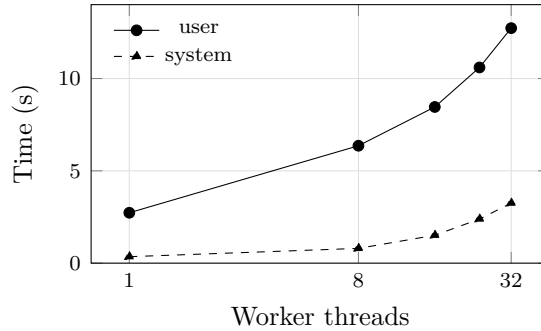
Figure 7: User and system time against worker count, for the runs of Table 14. Across a 32\times increase in workers user time rises by 4.7\times while system time rises by 9\times . System time is the faster-growing term and it tracks the resident set, so what the efficiency decline of Figure 8 is spent on is memory acquisition rather than lock contention.
