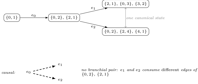
Figure 1: Two steps of \{x, y\} \rightarrow \{x, z\}, \{z, y\} from a single edge, as the engine reports them. Four raw states become three canonical ones: the two depth-2 results are isomorphic and are identified. Both causal edges descend from e_0 , because each depth-2 event consumes one of the two edges e_0 produced. The branchial relation is empty: e_1 and e_2 share an input state, which resembles a sibling pair, but branchial edges connect co-consumers of a common edge and these consume different ones. Every element is drawn from the engine’s own output.
