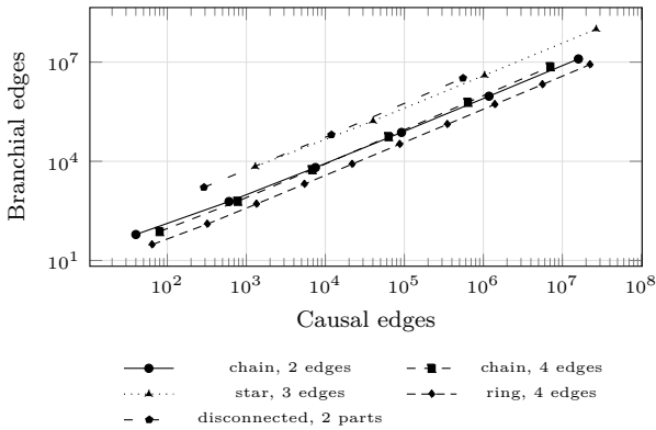
(b) Branchial edges against causal edges, both logarithmic; every point is one (shape, depth) run.
