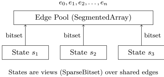
Figure 3: Unified edge storage with state views
