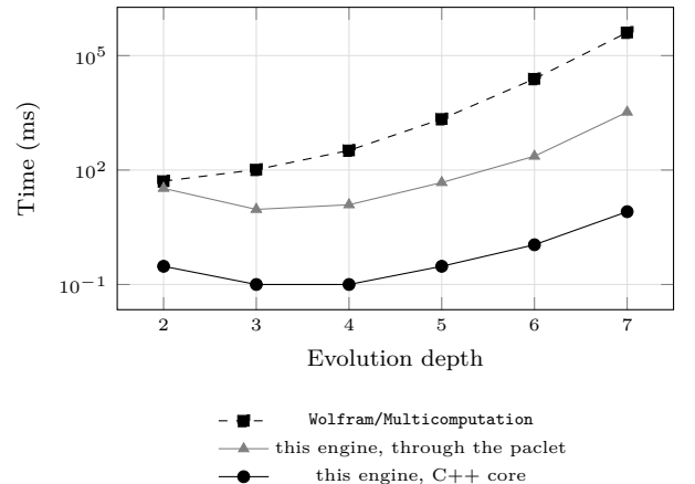
Figure 4: Evolution time against depth on the same rule and initial condition, all three series computing identical state and causal-edge counts at every depth: the authority, the engine through the packet, and the engine’s C++ core. The outer gap is the speedup of Table 5; the inner gap is the Wolfram layer alone.
