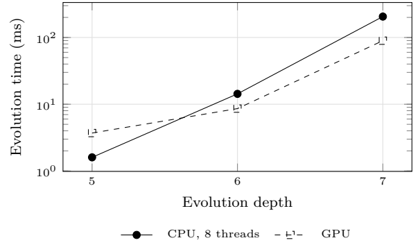
(a) Evolution time against depth, the device against eight CPU threads (Table 7).
