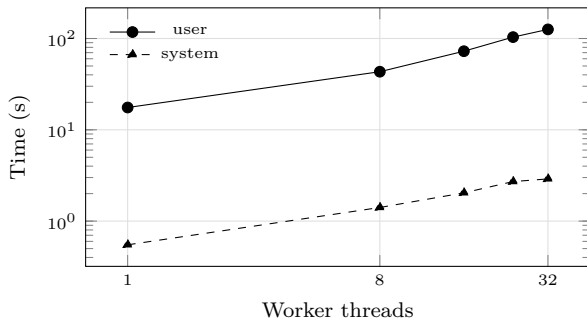
Figure 6: User and system time against worker count, for the runs of Table 13: across a 32× increase in workers, user time rises by 7.2× and system time, thirty to forty-five times smaller, by 5×.
