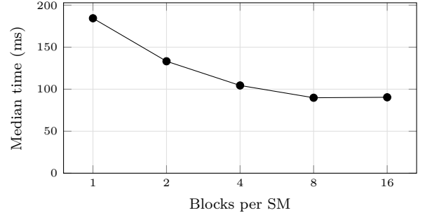
(b) Median time against the resident kernel’s grid size (Table 14).
