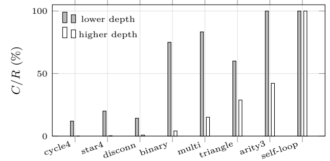
Figure 2: C/R , the ceiling of Proposition 3.3 on the fraction of IR invocations a pre-filter could elide, for each corpus case at two depths. Every case that continues to rewrite decreases; a case that does not is one that reaches a fixed point before the higher depth, as self-loop does after one event, with a ratio of 100% at both depths. Values as in Table 1.
