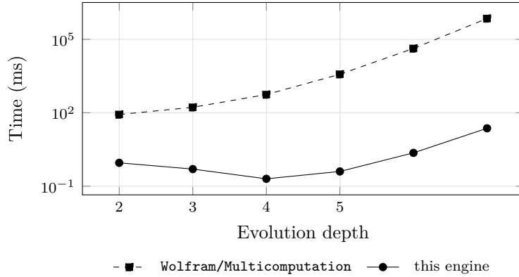
Figure 5: Evolution time against depth for the two implementations, logarithmic in time, on the same rule and initial condition and producing identical state and causal-edge counts at every depth. The vertical separation is the speedup reported in Table 6: 2,770\times at depth 4, rising to 30,627\times at depth 7. The depth-2 point includes one-time initialization on the Wolfram side, and this engine’s times at depths 3–5 are near the timer’s resolution.
