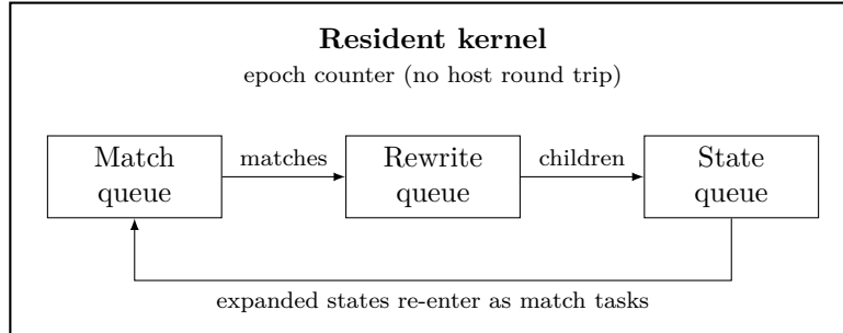
Figure 4: Queue structure of the resident device kernel. Work circulates between the three queues without returning to the host; an epoch counter separates evolution steps.
