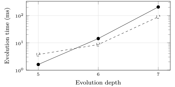
(a) Evolution time against depth, the device against eight CPU threads (Table 9).
