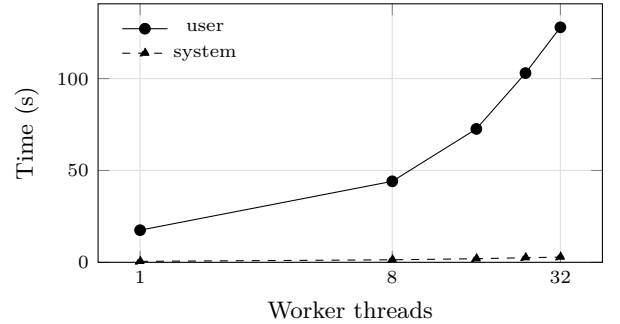
Figure 7: User and system time against worker count, for the runs of Table 14. Across a 32× increase in workers user time rises by 7.3× while system time rises by 5×. System time is two orders of magnitude the smaller and tracks the fault count. The efficiency decline of Figure 8 is spent in user time, on cross-domain data flow (Table 14’s section), with memory acquisition a minor kernel-side term.
