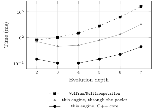
Figure 4: Evolution time against depth for MultwaySystem , the engine through the packet, and the engine’s C++ core, on the same rule and initial state; all three give the same state and causal-edge counts at every depth. The gap between the first and last series is the speedup of Table 4; the gap between the last two is the cost of the Wolfram interface.
