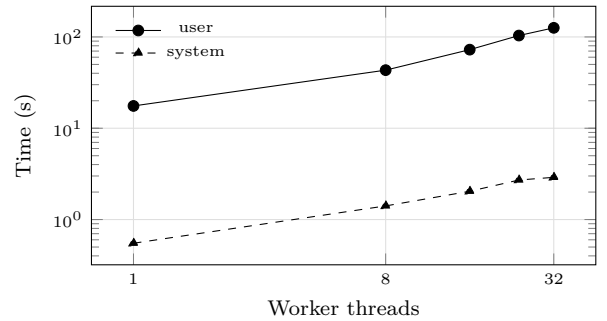
Figure 6: User and system time against worker count, for the runs of Table 12: across a 32× increase in workers, user time grows 7.2× and system time, thirty to forty-five times smaller, grows 5×.
