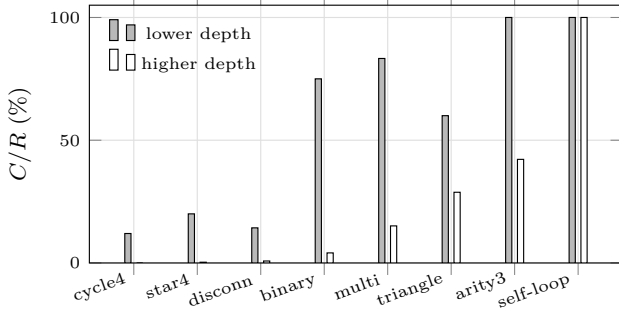
Figure 2: C/R for each corpus workload at two depths: the upper bound of Proposition 3.3 on the fraction of IR calls a pre-filter can skip. It falls with depth on every workload that keeps rewriting. self-loop reaches a fixed point after one event and stays at 100%. Values as in Table 1.
