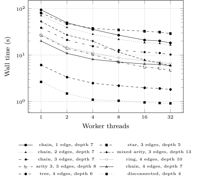
Figure 7: Wall time against worker count for the sweep’s ten timed workloads, each at the depth its legend entry states. Both axes are logarithmic; the legend lists the curves in descending order of single-threaded time.
