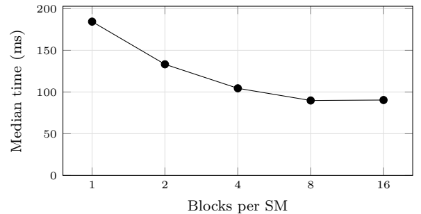
(b) Median time against the resident kernel’s grid size (Table 13).
