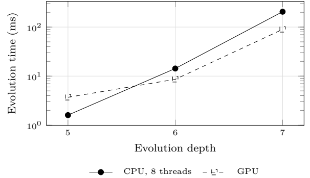
(a) Evolution time against depth, the device against eight CPU threads (Table 6).
