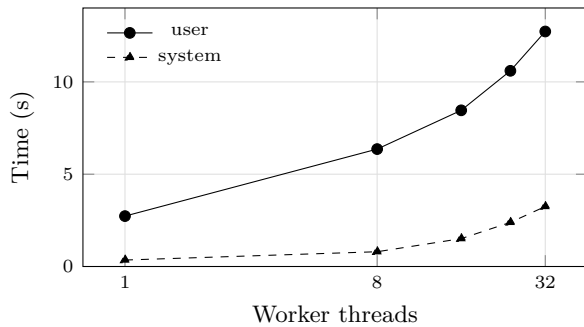
Figure 7: User and system time against worker count, for the runs of Table 14. Across a 32\times increase in workers user time rises by 4.7\times while system time rises by 9\times . System time is the faster-growing term and it tracks the resident set, so what the efficiency decline of Figure 8 is spent on is memory acquisition rather than lock contention.
