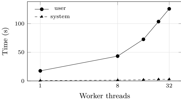
Figure 7: User and system time against worker count, for the runs of Table 14. Across a 32× increase in workers user time rises by 7.2× while system time rises by 5×. System time is thirty to forty-five times the smaller and tracks the fault count. The efficiency decline of Figure 8 is spent in user time, on cross-domain data flow (Table 14’s section), with memory acquisition a minor kernel-side term.
