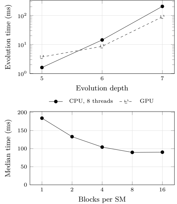
Figure 6: Left: evolution time against depth for the GPU and for eight CPU threads. The device is slower at depth five, where the work per launch does not amortize the launch cost, and faster from depth six. Right: median time against the resident kernel’s grid size. Time ceases to improve beyond eight blocks per streaming multiprocessor, which is the shipped default. Both panels plot the values of Tables 8 and 15, which carry the provenance of each measurement.
