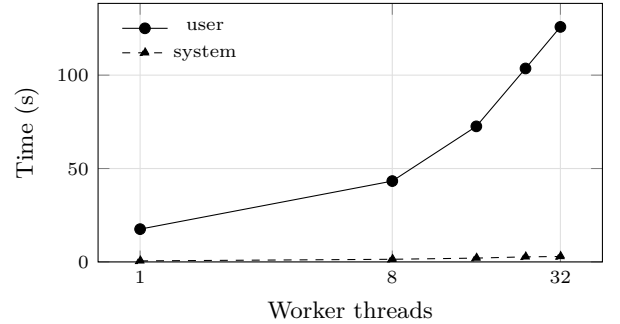
Figure 7: User and system time against worker count, for the runs of Table 14. Across a 32× increase in workers user time rises by 7.2× while system time rises by 5×. System time is thirty to forty-five times the smaller and tracks the fault count. The efficiency decline of Figure 8 is spent in user time, on cross-domain data flow (Table 14’s section), with memory acquisition a minor kernel-side term.
