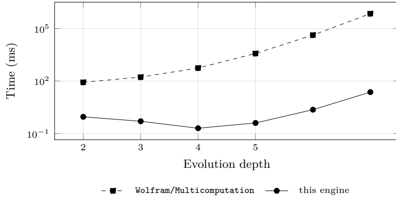
Figure 5: Evolution time against depth for the two implementations, logarithmic in time, on the same rule and initial condition and producing identical state and causal-edge counts at every depth. The vertical separation is the speedup reported in Table 6: 2,770\times at depth 4, rising to 30,627\times at depth 7. The depth-2 point includes one-time initialization on the Wolfram side, and this engine’s times at depths 3–5 are near the timer’s resolution.
