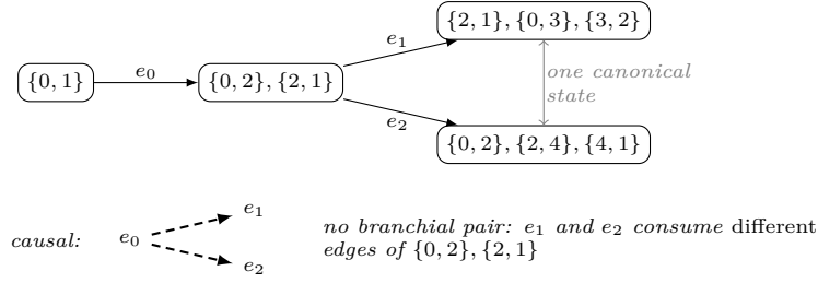
Figure 1: Two steps of \{x, y\} \rightarrow \{x, z\}, \{z, y\} from a single edge, exactly as the engine reports it. Four raw states become three canonical ones: the two depth-2 results are isomorphic and are identified. Both causal edges descend from e_0 , because each depth-2 event consumes one of the two edges e_0 produced. The branchial relation is empty here, and for a reason worth stating: e_1 and e_2 share an input state, which resembles a sibling pair, but branchial edges connect co-consumers of a common edge and these consume different ones. Every element is output of canonical_causal_oracle --dump 2 .
