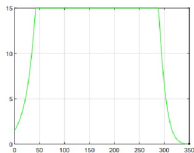
Escenario 1B: u_{\max} = 15, T^* = 350 days
