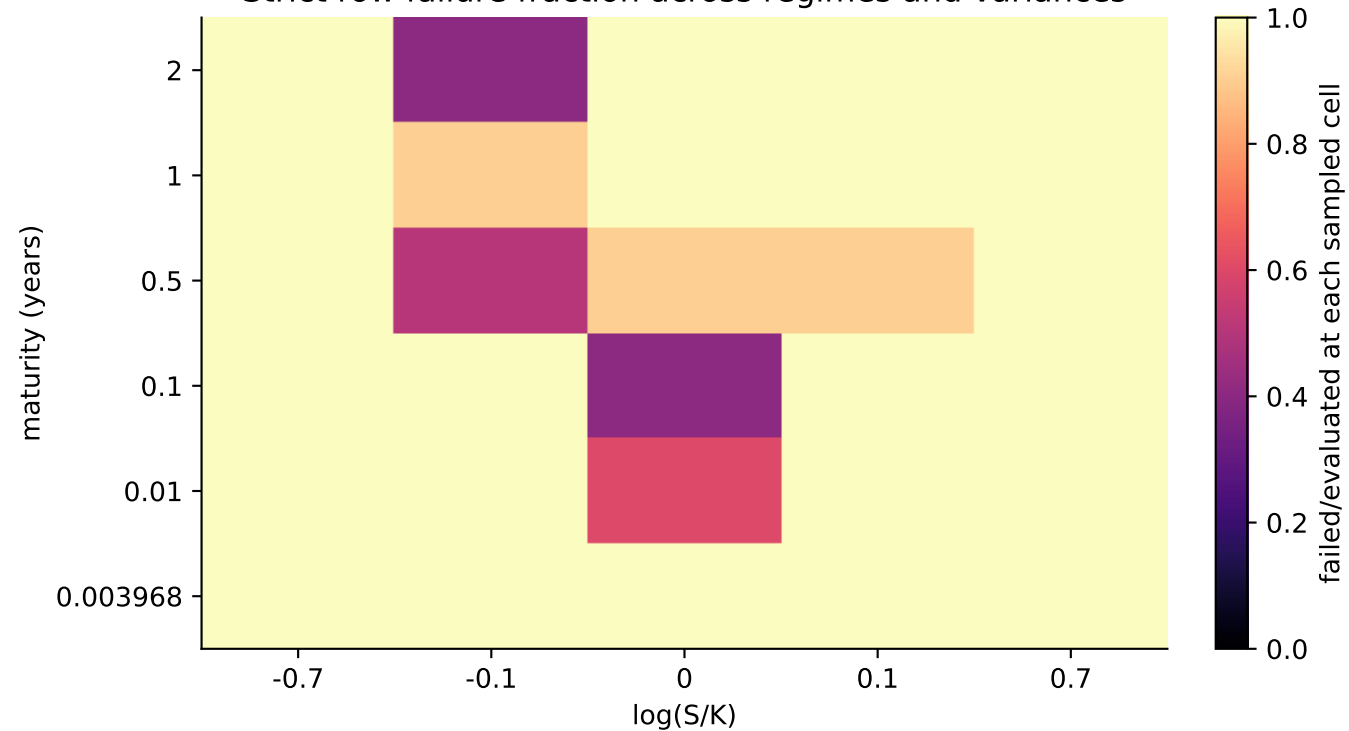
Strict row failure fraction across regimes and variances
