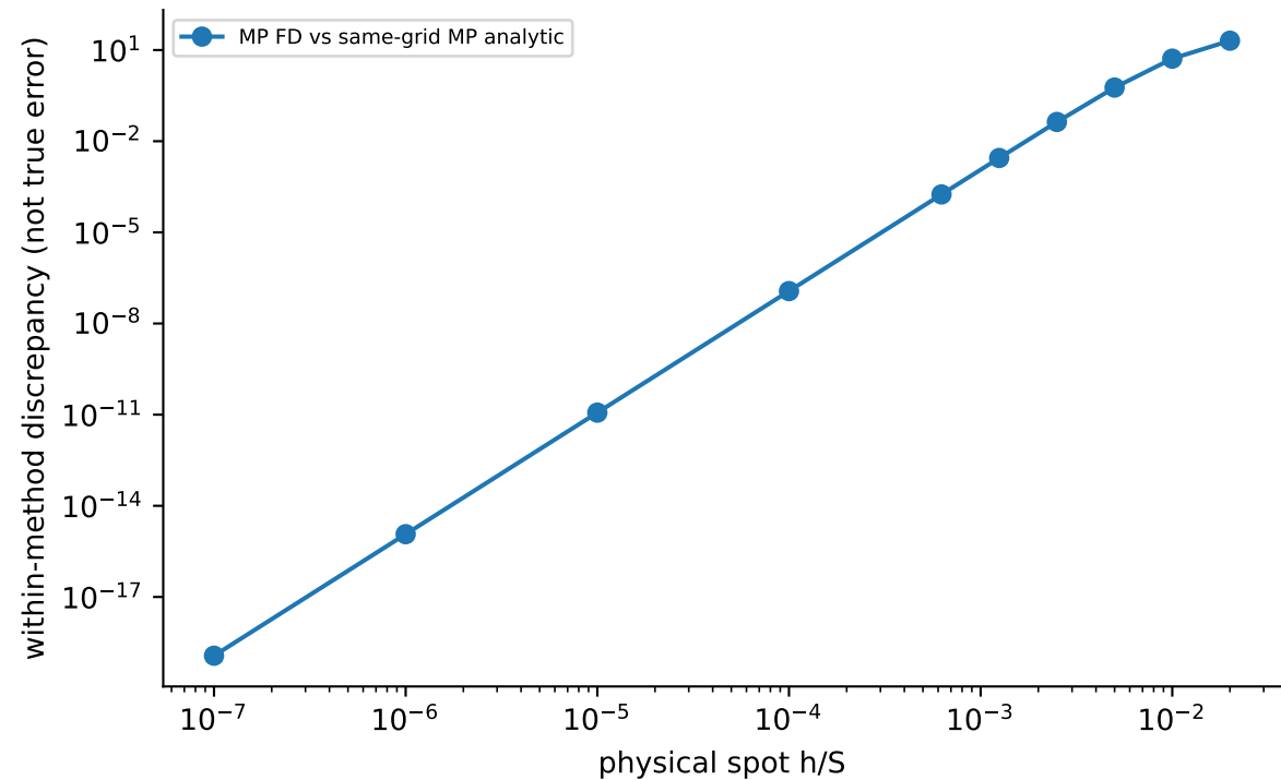
GREEK_PRIORITY_0_R0; MP U=8192, dps=80
