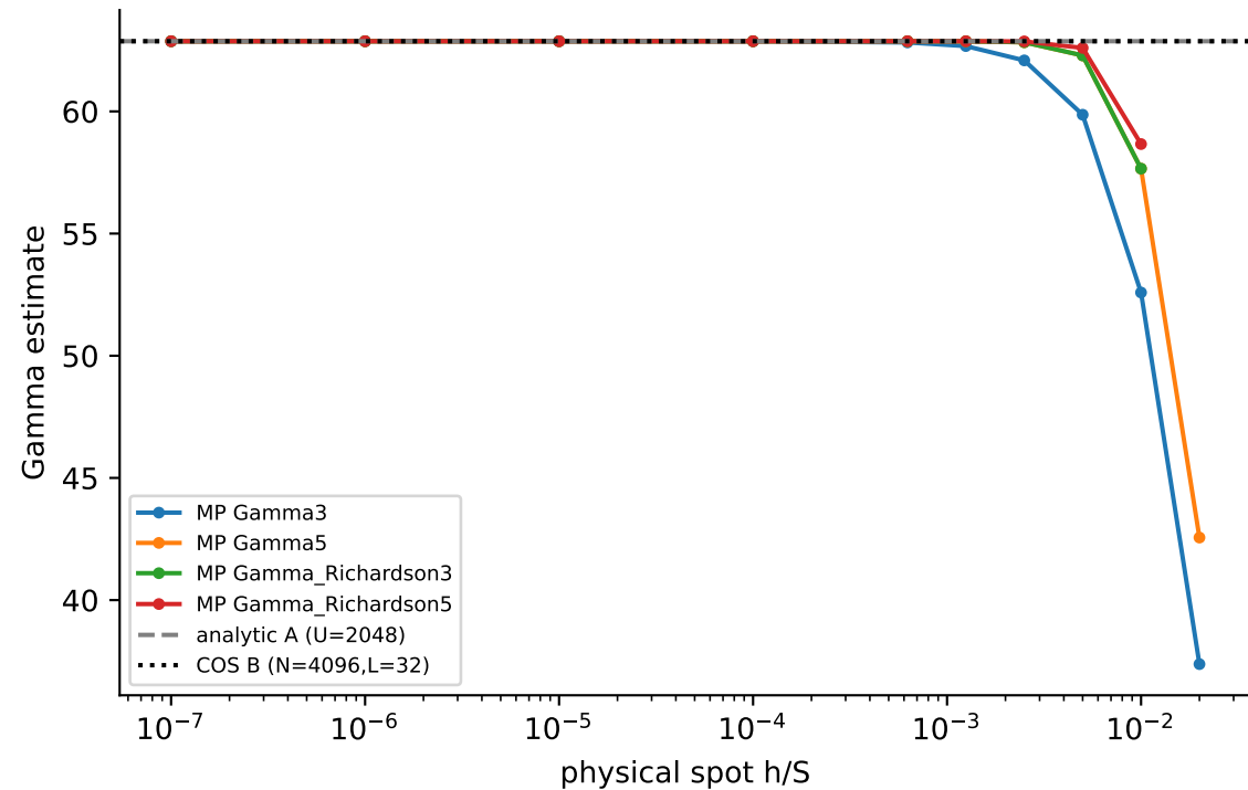
GREEK_PRIORITY_0_R0; MP U=8192, dps=80
