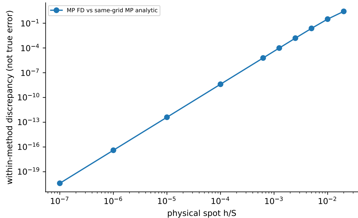
GREEK_PRIORITY_11_R3; MP U=8192, dps=80
