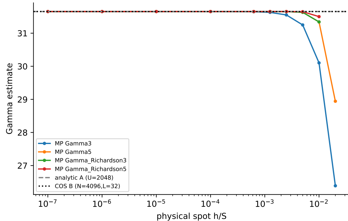
GREEK_PRIORITY_11_R3; MP U=8192, dps=80
