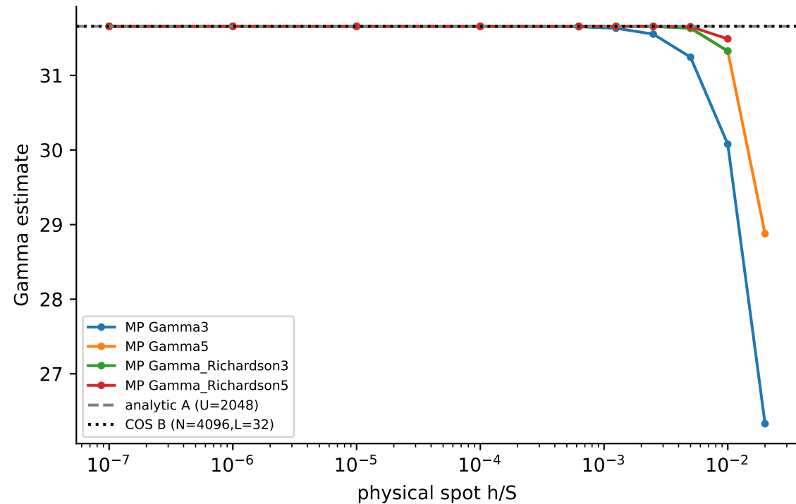
GREEK_PRIORITY_14_R5; MP U=8192, dps=80
