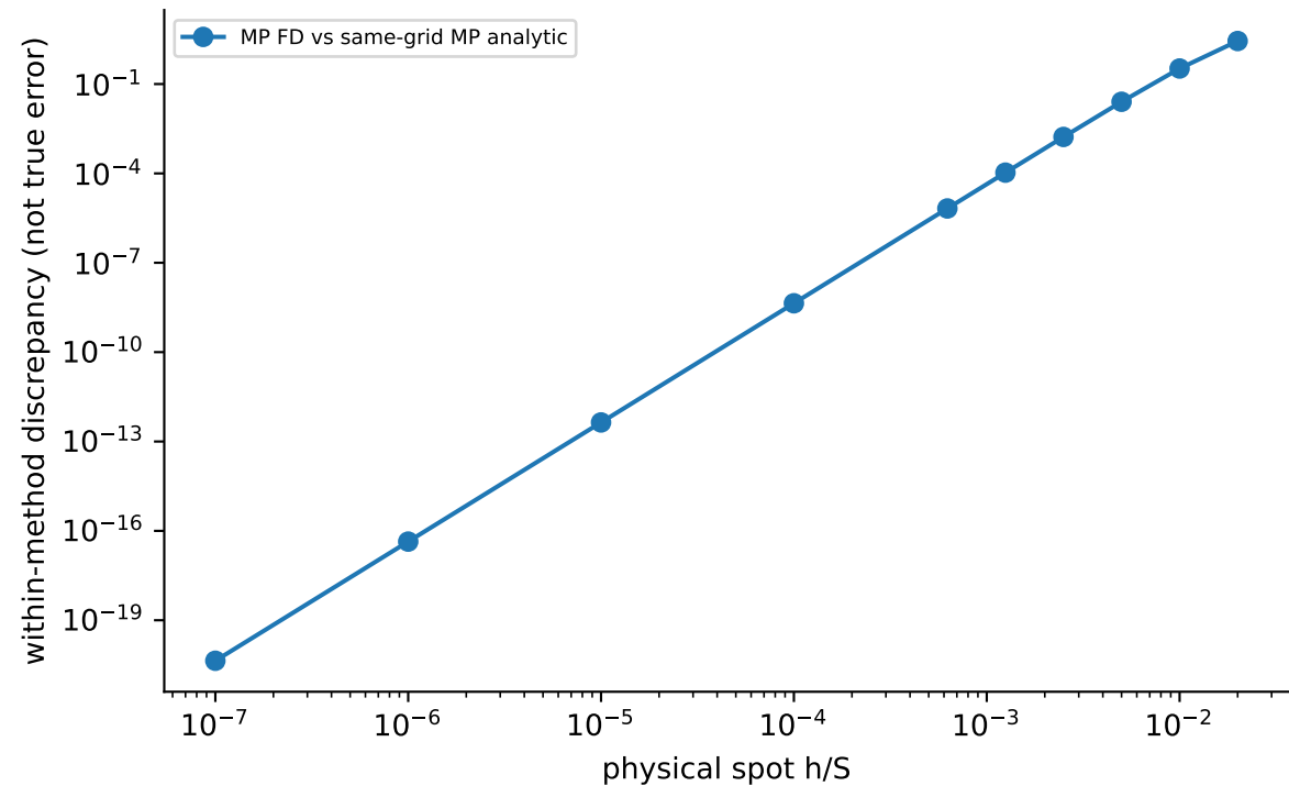
GREEK_PRIORITY_14_R5; MP U=8192, dps=80
