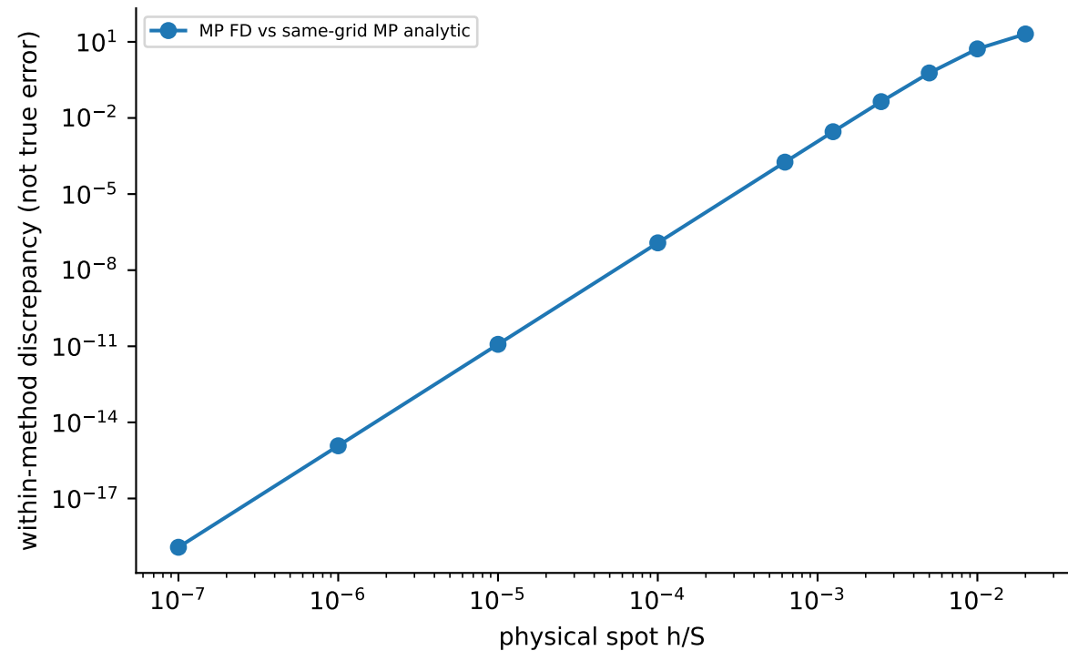
GREEK_PRIORITY_3_R1; MP U=8192, dps=80
