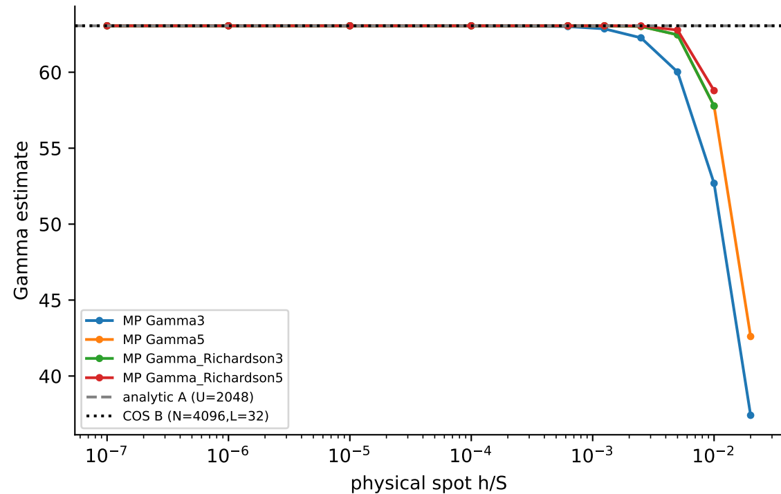
GREEK_PRIORITY_3_R1; MP U=8192, dps=80
