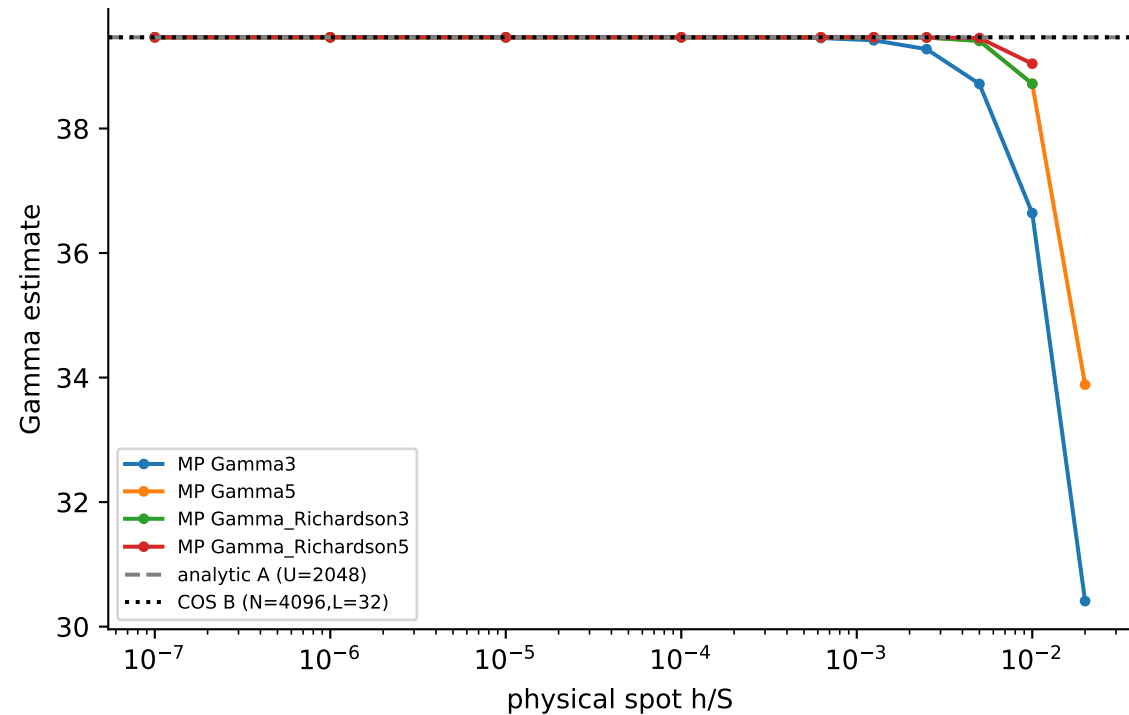
GREEK_PRIORITY_4_R1; MP U=8192, dps=80
