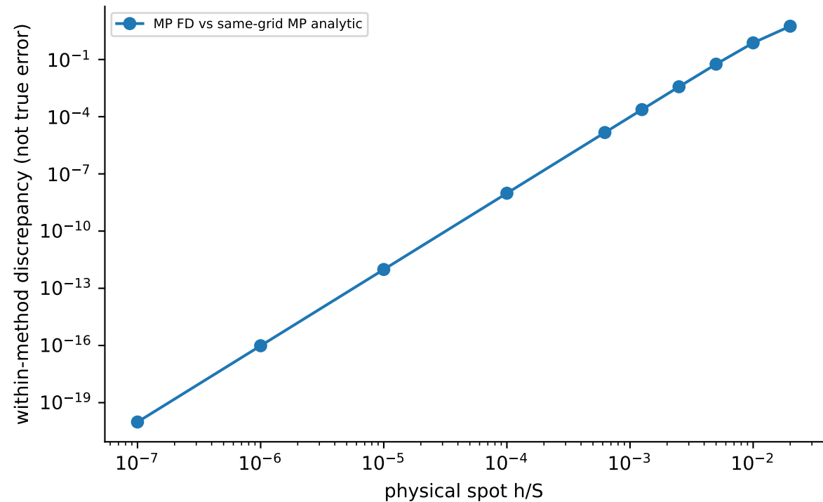
GREEK_PRIORITY_4_R1; MP U=8192, dps=80
