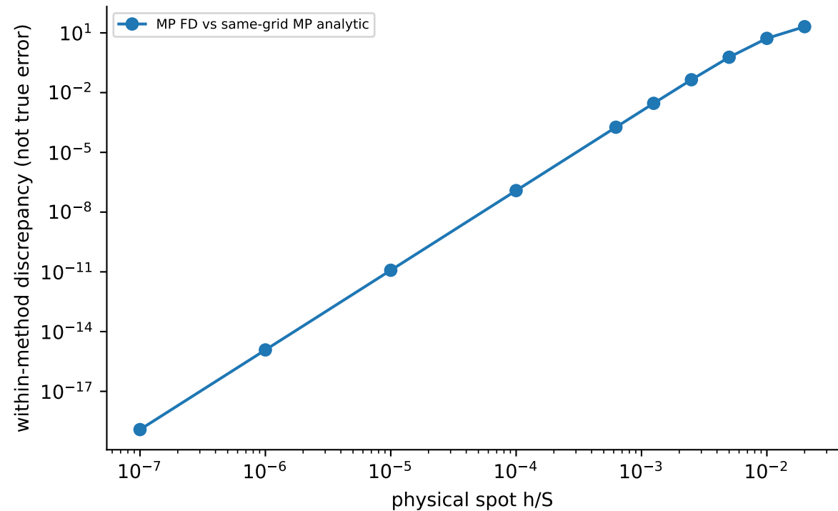
GREEK_PRIORITY_6_R2; MP U=8192, dps=80
