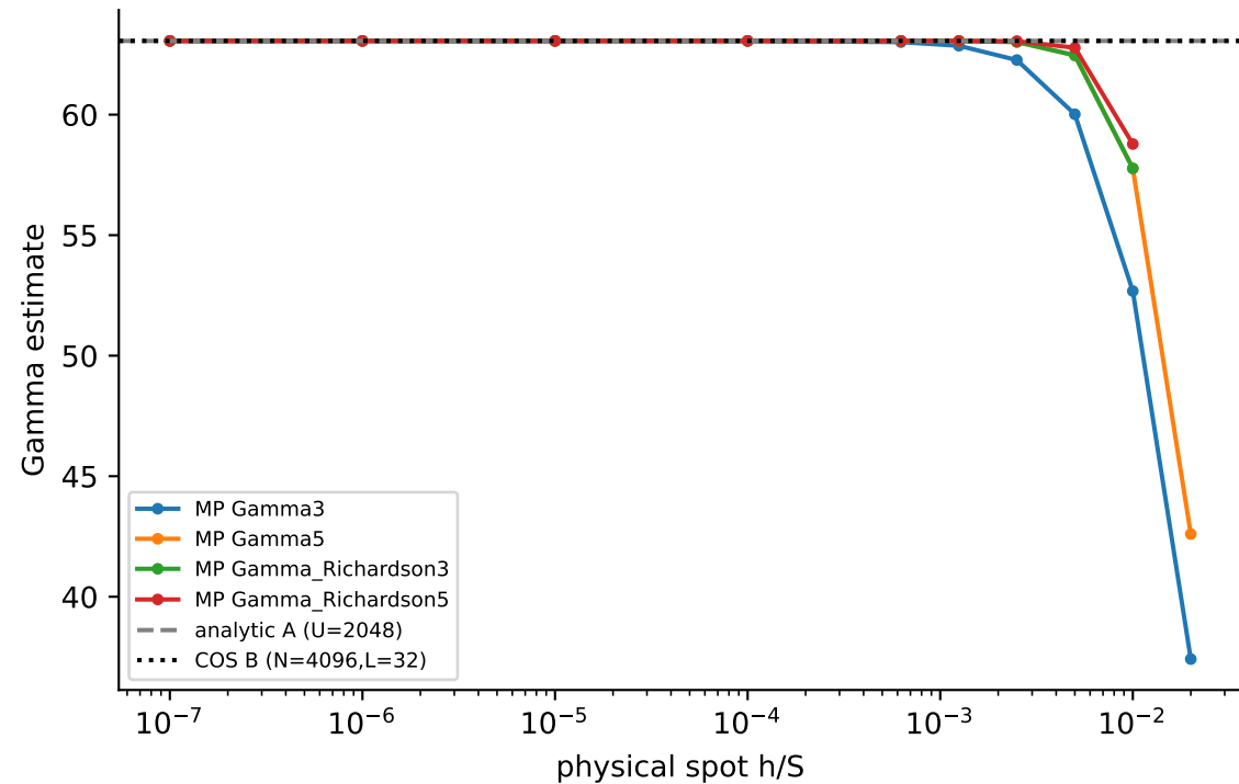
GREEK_PRIORITY_6_R2; MP U=8192, dps=80
