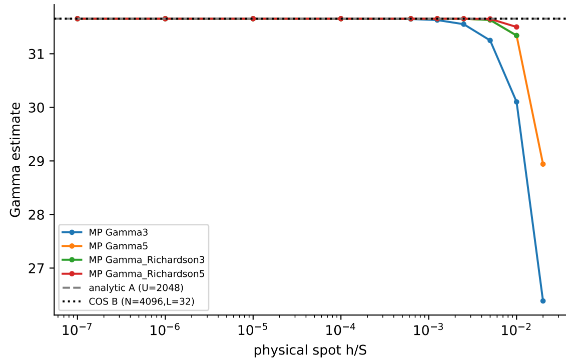
GREEK_PRIORITY_8_R2; MP U=8192, dps=80
