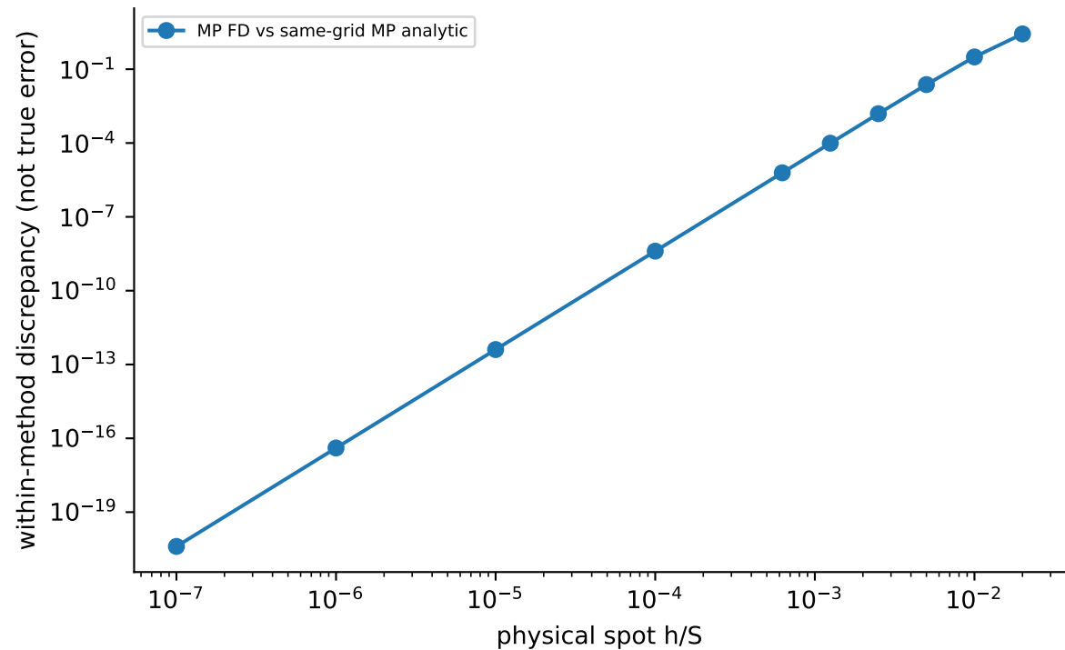
GREEK_PRIORITY_8_R2; MP U=8192, dps=80
