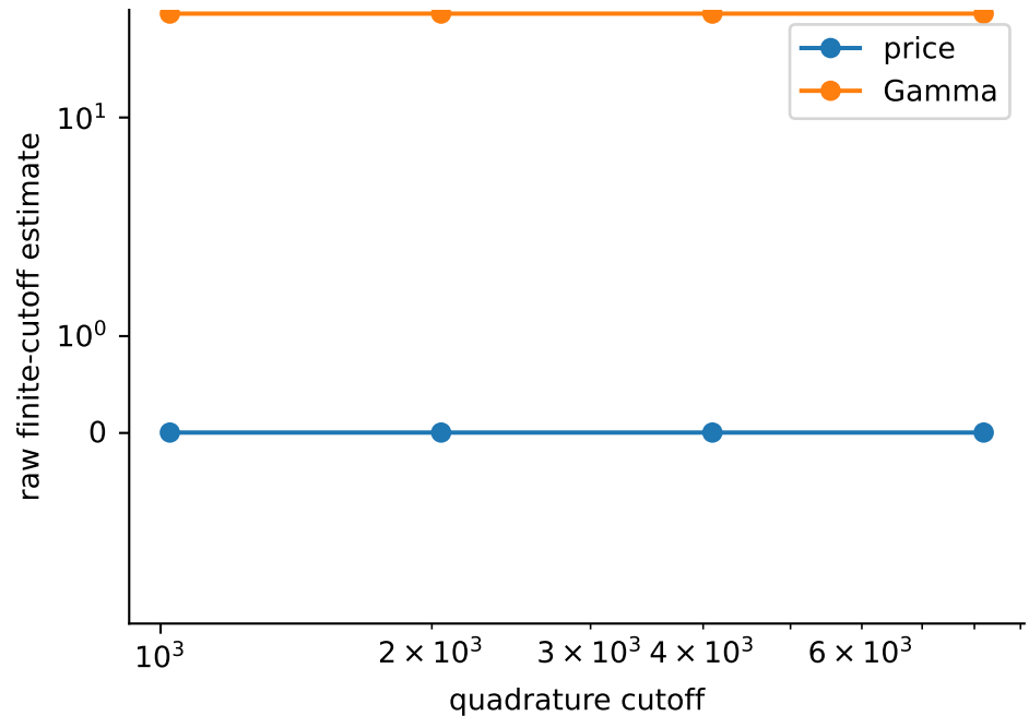
GREEK_PRIORITY_10_R3: digit agreement does not certify the integration tail
