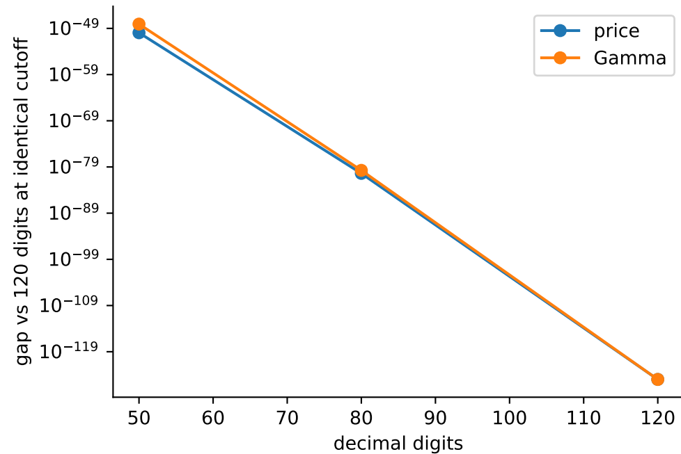
GREEK_PRIORITY_10_R3: digit agreement does not certify the integration tail
