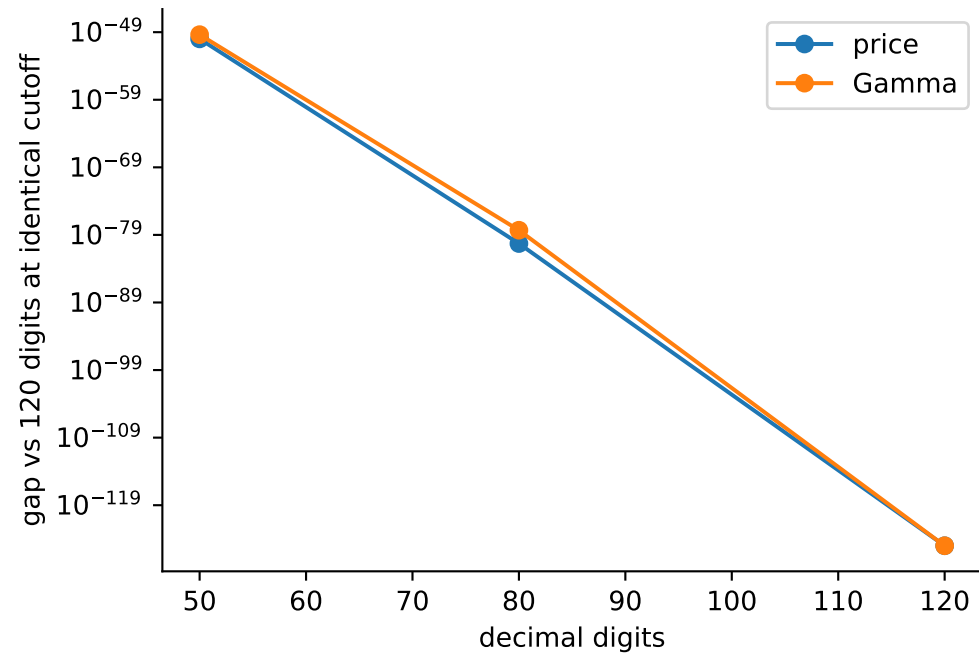
GREEK_PRIORITY_11_R3: digit agreement does not certify the integration tail
