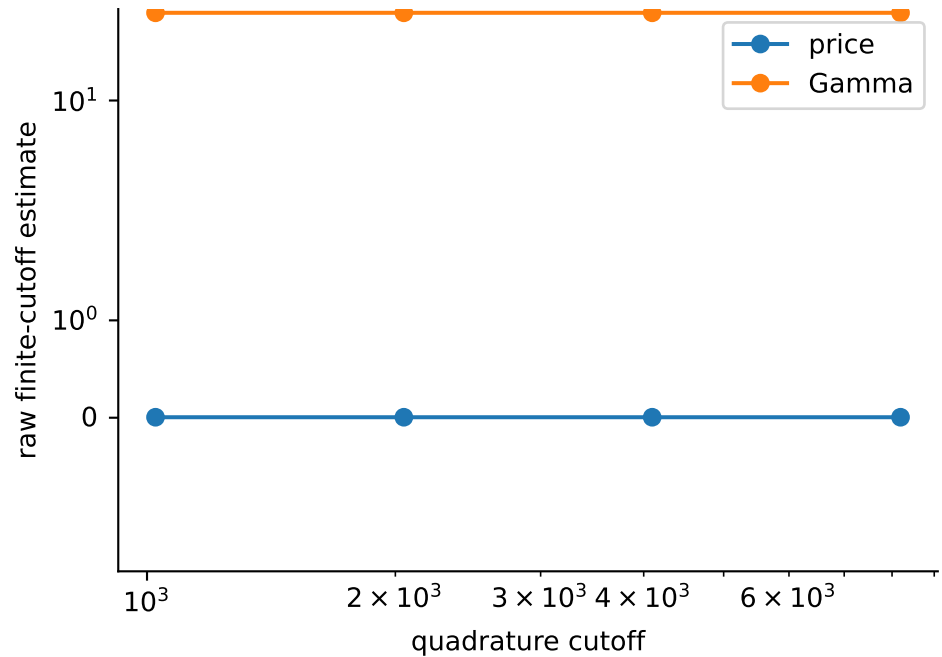
GREEK_PRIORITY_11_R3: digit agreement does not certify the integration tail
