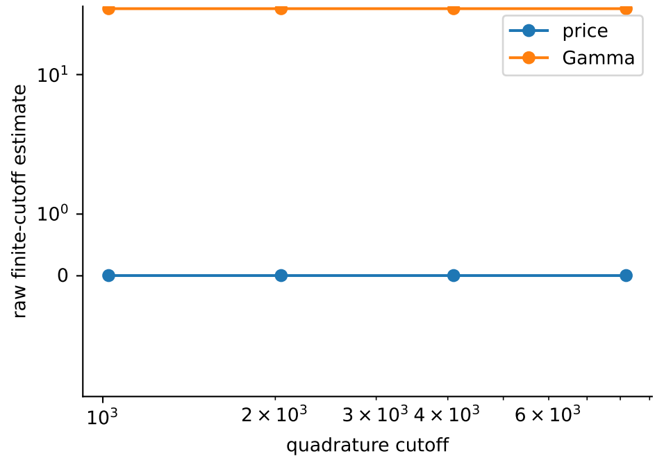
GREEK_PRIORITY_1_R0: digit agreement does not certify the integration tail
