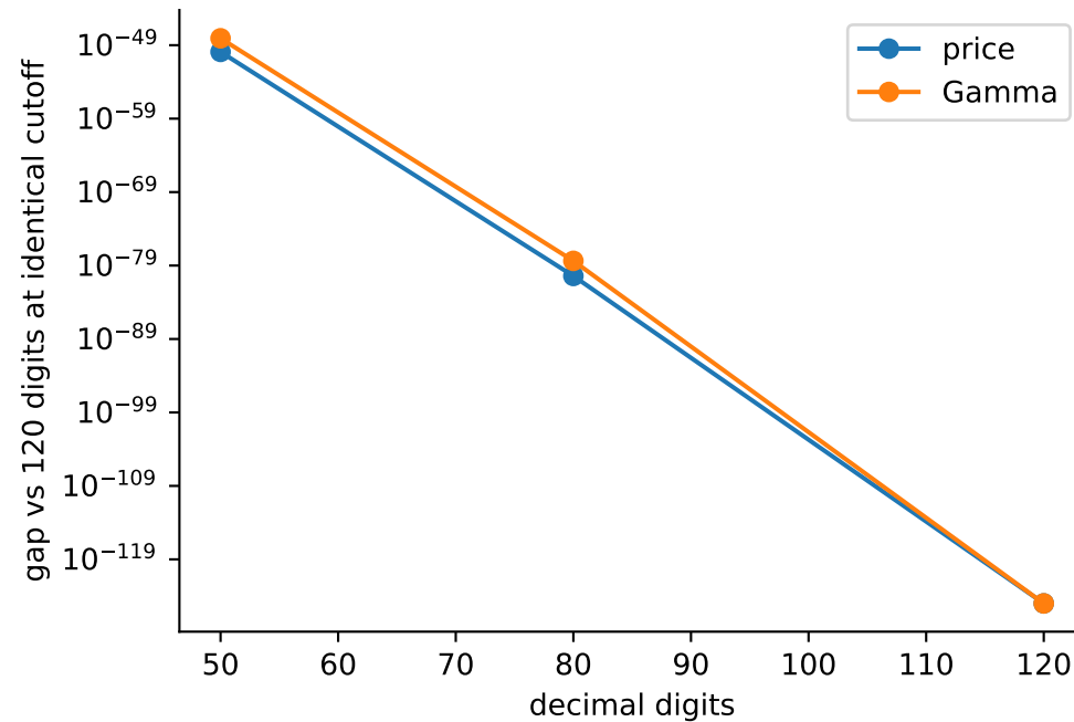
GREEK_PRIORITY_1_R0: digit agreement does not certify the integration tail
