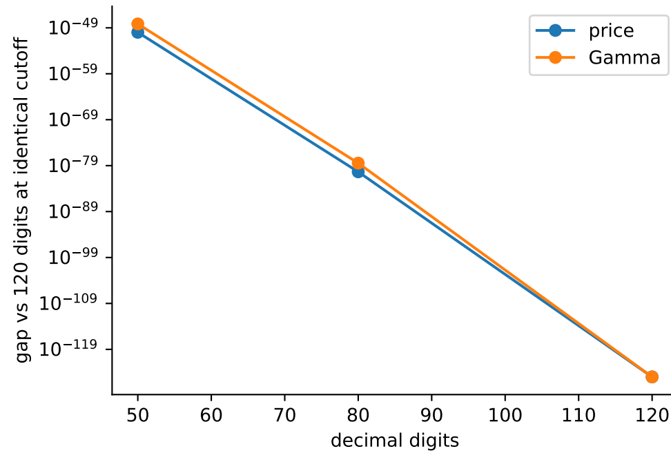
GREEK_PRIORITY_7_R2: digit agreement does not certify the integration tail
