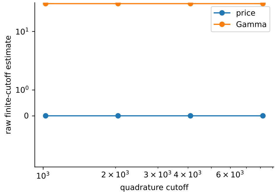
GREEK_PRIORITY_7_R2: digit agreement does not certify the integration tail
