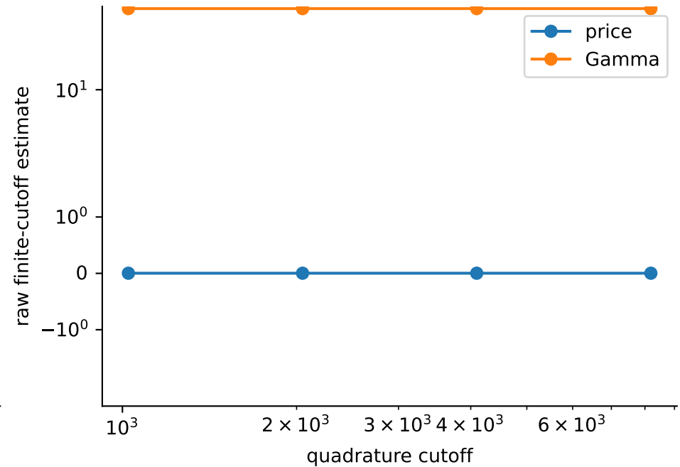
GREEK_PRIORITY_9_R3: digit agreement does not certify the integration tail
